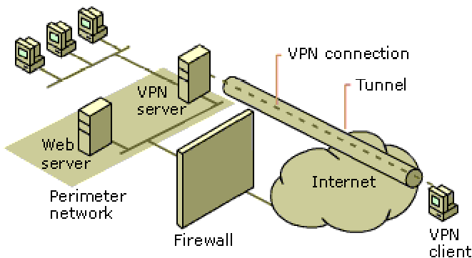
Figure 4 The VPN server behind the firewall on the perimeter network
