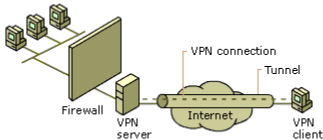
Figure 3 The VPN server in front of the firewall
