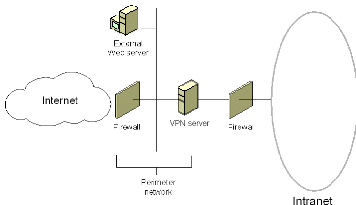
Figure 5 The VPN server between two firewalls on the perimeter network
