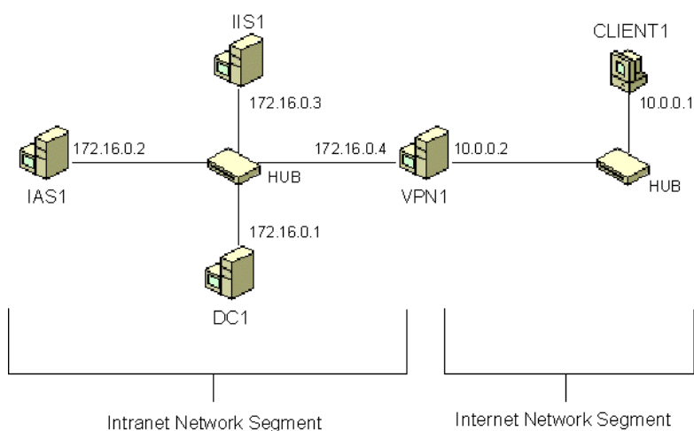
Figure 7. Configuration of the VPN test lab
